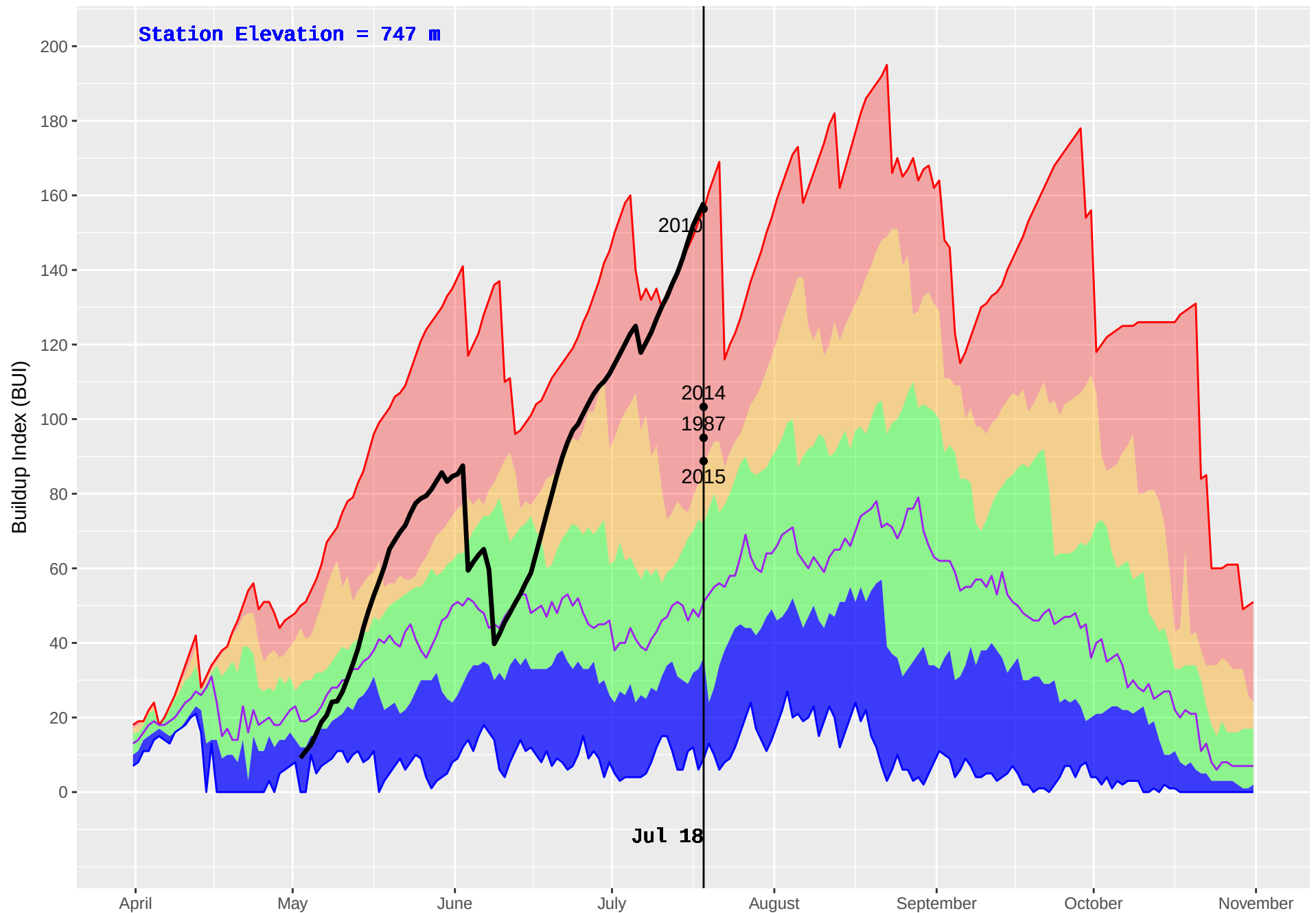
PEDEN (178) : Historical (1984–2016) and Current (2018) Daily Buildup Index (BUI)
