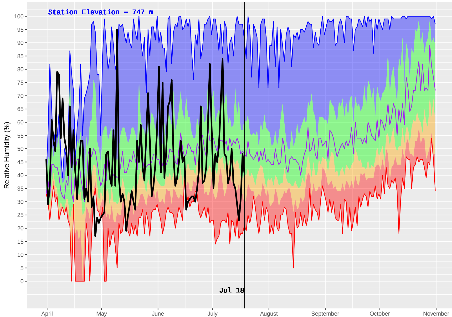
PEDEN (178) : Historical (1984–2016) and Current (2018) Daily Relative Humidity
