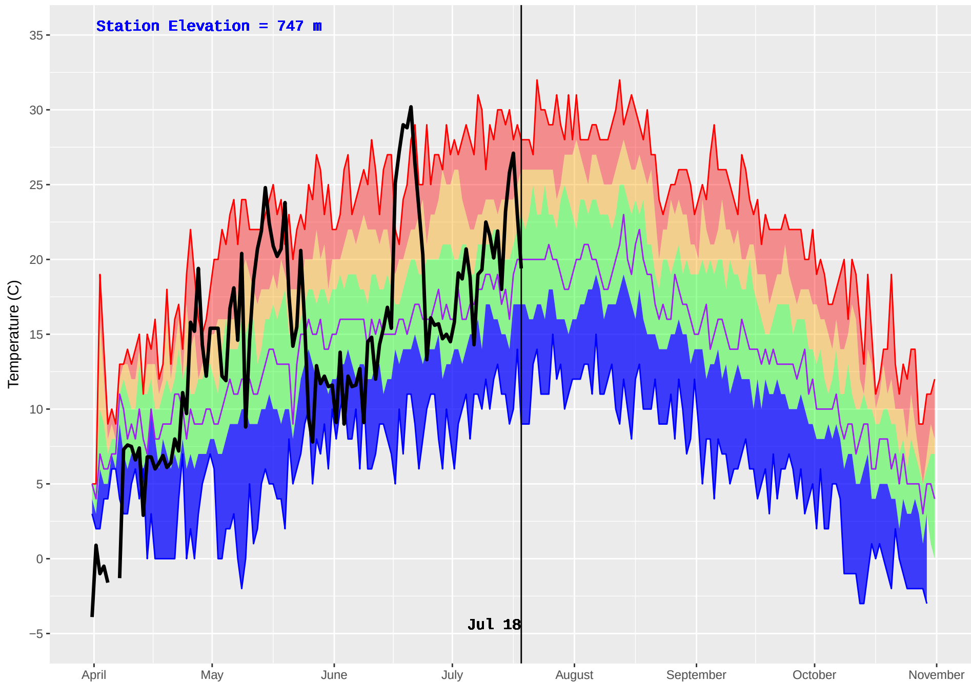
PEDEN (178) : Historical (1984–2016) and Current (2018) Daily Temperature
